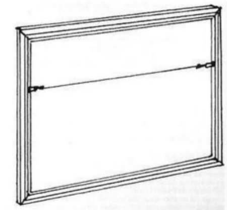
Fig 7. Tight tension wire, one third of the way below the top of the canvas, with wire not less than 8 cm from top.
